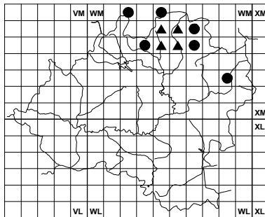
Mercurialis perennis
