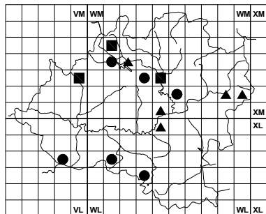
Myosotis discolor
